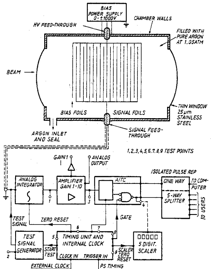
Fig. 5 SIMPLIFIED DIAGRAM OF THE ARGONION AND ITS INTERCONNECTIONS WITH THE ASSOCIATED ELECTRONICS
