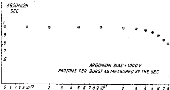
Fig. 4 LINEARITY OF THE ARGONION
