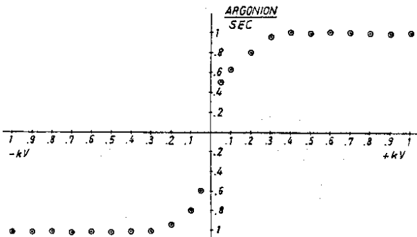
Fig. 3 BIAS CURVE OF THE ARGONION OBTAINED WITH BEAM INT. \sim 10^{11} PROTONS PER BURST
