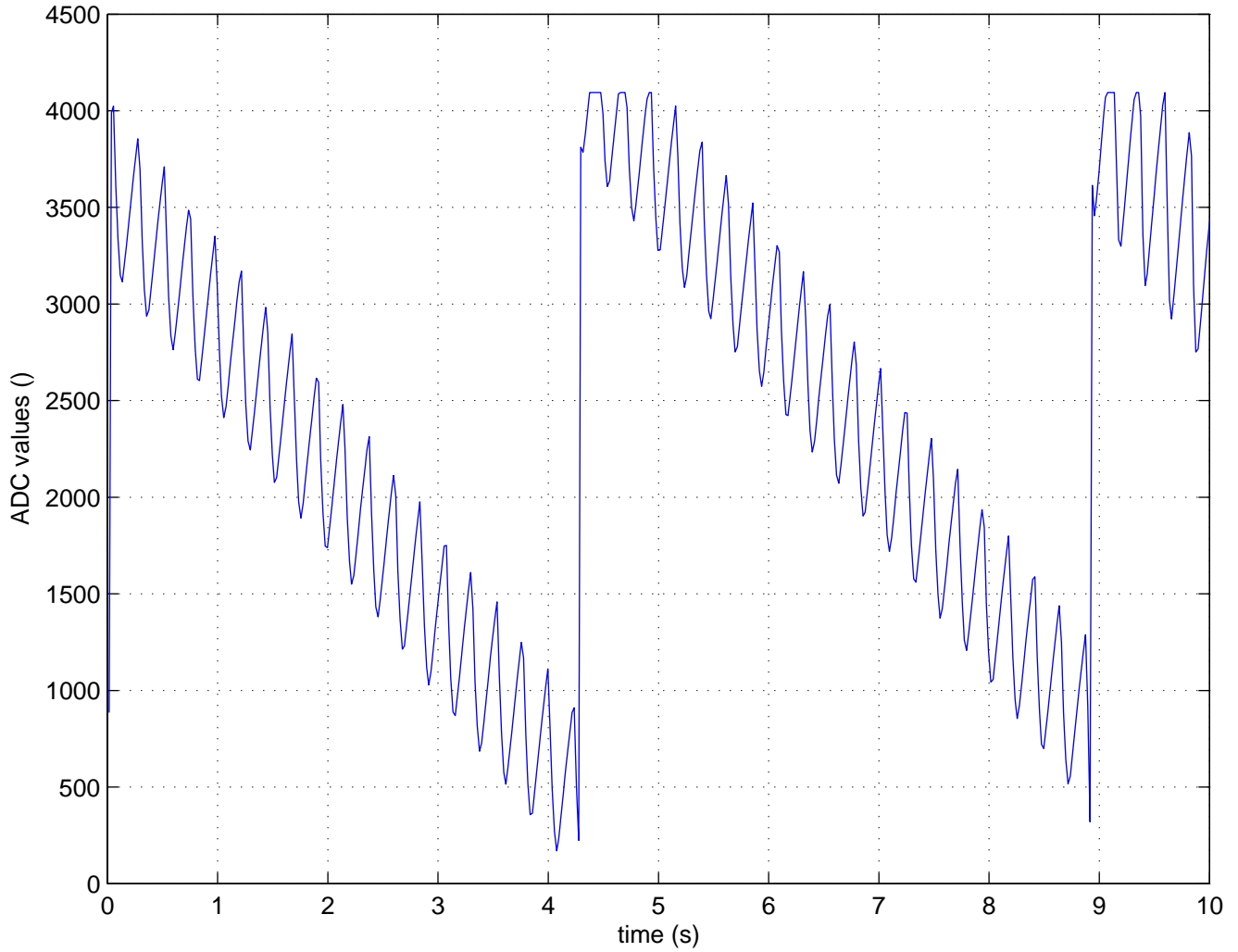
ADC values when a modulation of the high voltage is applied
