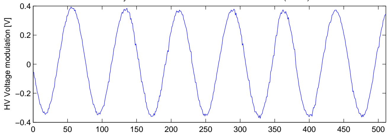
Very Low Level Modulation 24bits ADC with filter (21bits)
