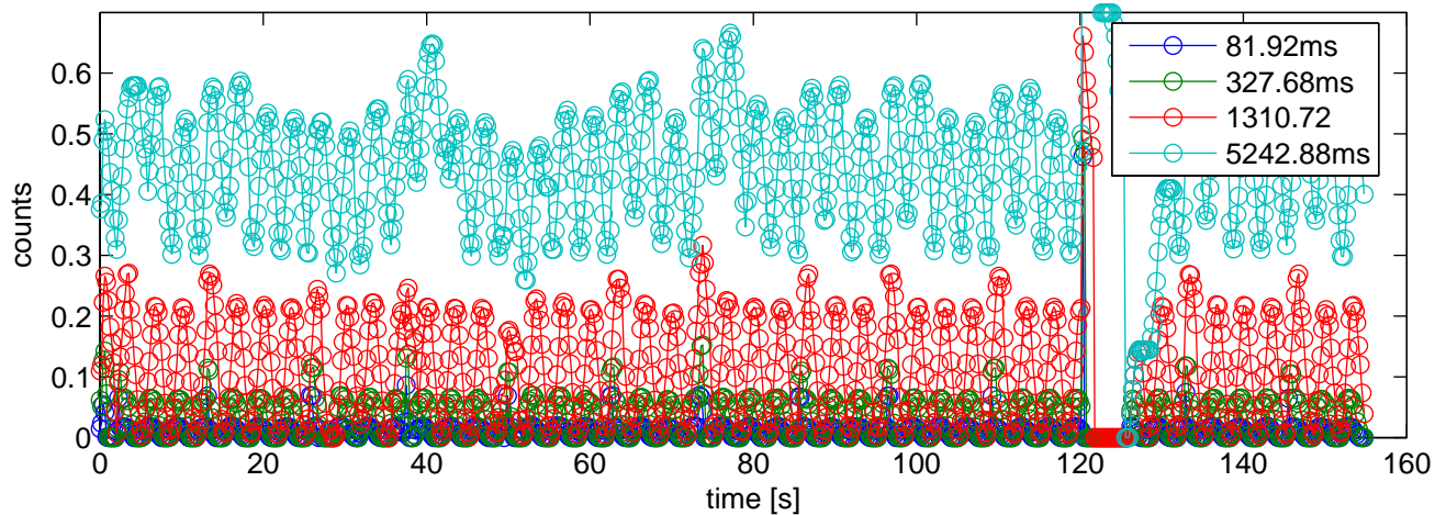
Low Voltage modulation at the HV input of a LHC BLM chamber
