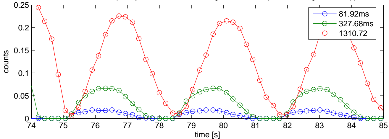
Parameters: frequency 300mHz, offset Voltage: 500mV, amplitude Voltage: 300mVpp
