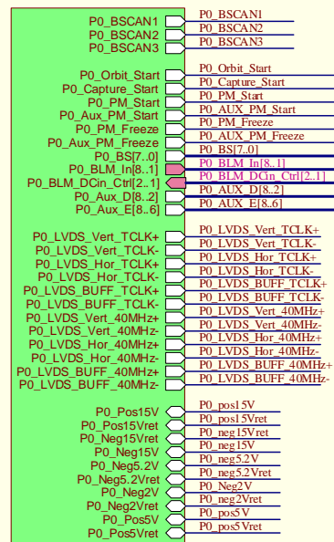
DAB64x_VME_P0_Connector.SchDoc
