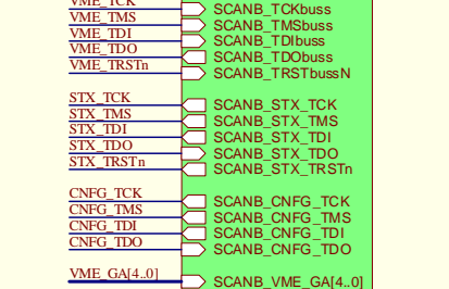
DAB64x_SCAN_Bridge.SchDoc
