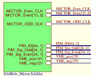
DAB64x_Mictor.SchDoc
