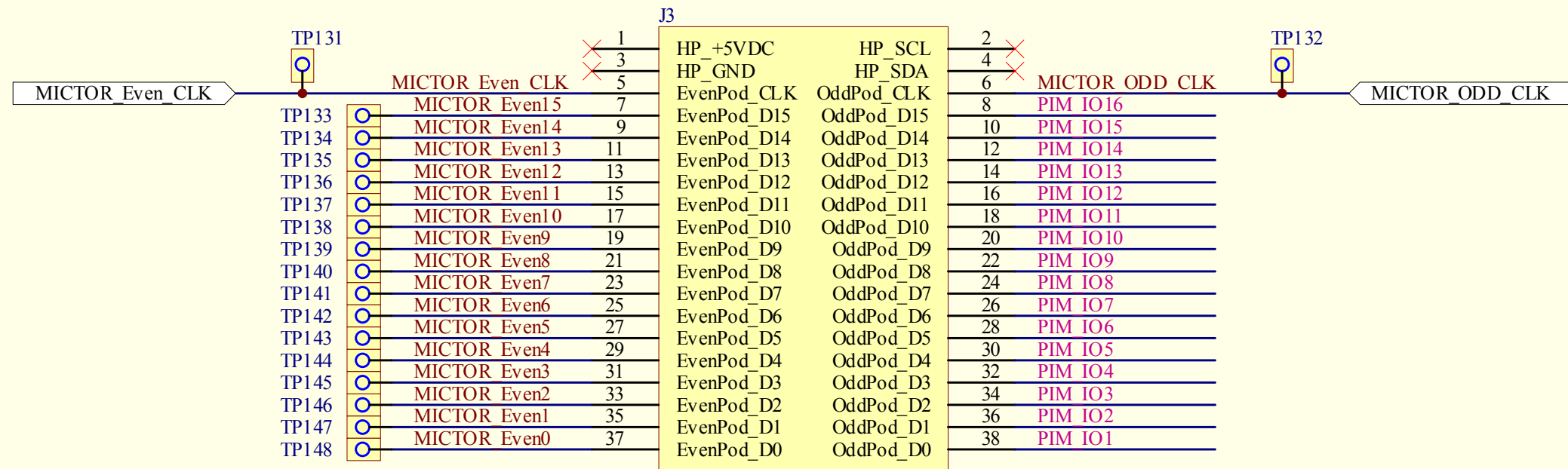
MICTOR 38 pin HP Probe
