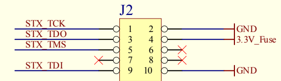
JTAG->STRATIX
