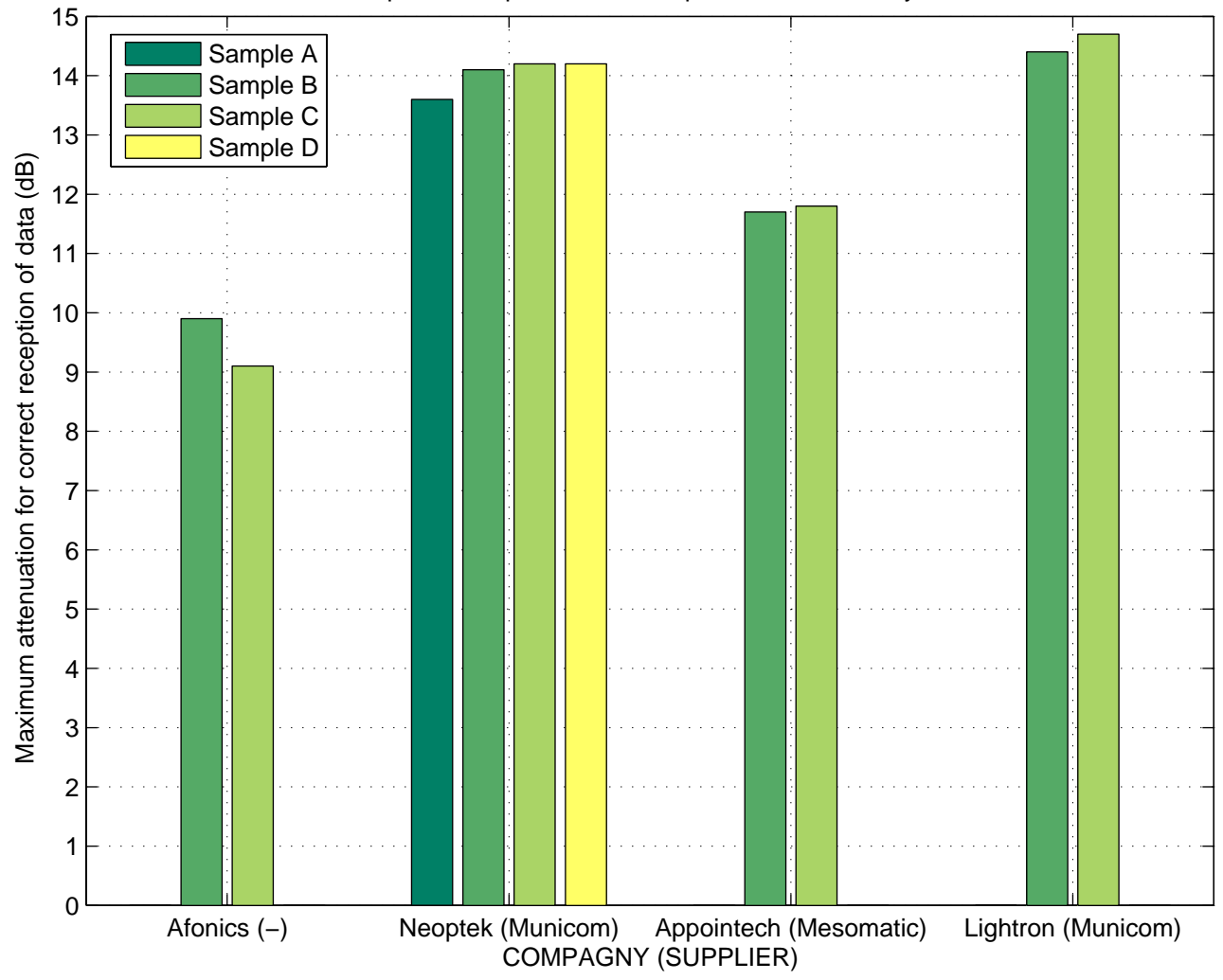
Comparison of photodiode samples with the BLM system
