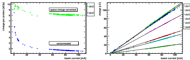
Figure 4: Signal as function of beam current at 920 GeV beam energy before (left) and after (right and left) space charge correction.
