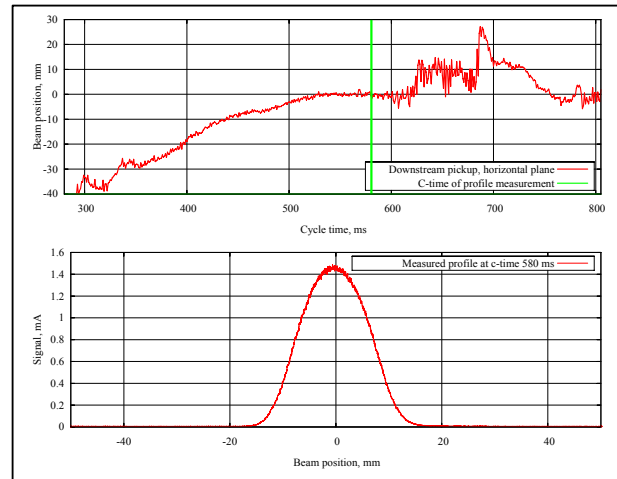
Figure 8: Horizontal profile measurement of a c entered beam in the PS booster: a) beam position from a downstream pickup, b) profile, measured by a wire scanner.
