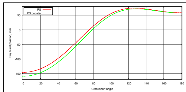
Figure 5: Lookup tables of theoretical projected positions.
