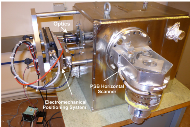
Figure 1: Calibration bench with a horizontal PS booster scanner
