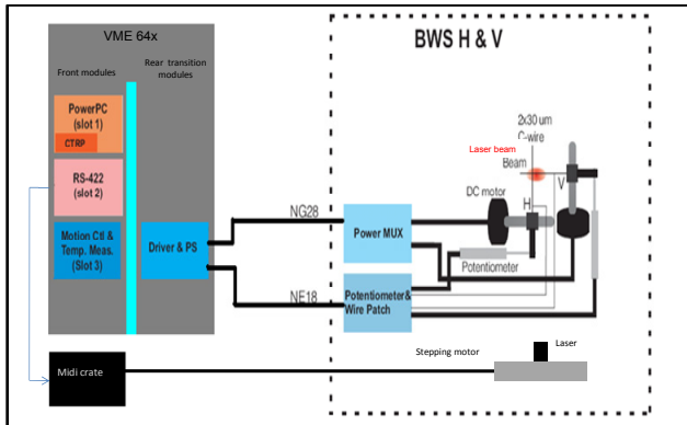
Figure 3: Electronics schematics of the calibration bench.
