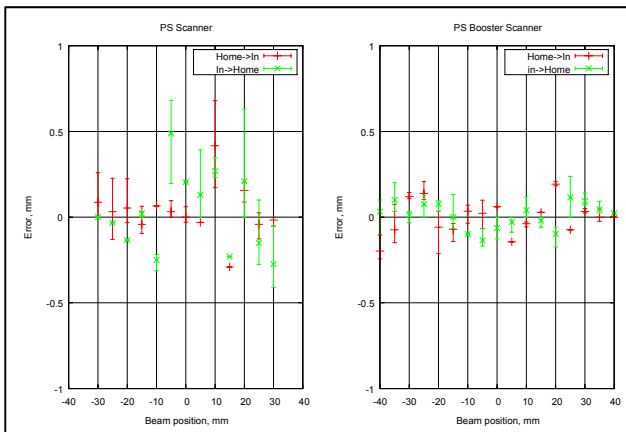
Figure 7: Check results of a scanner in PS domain and a scanner in PS booster domain. The wire speed is 15 m/s.
