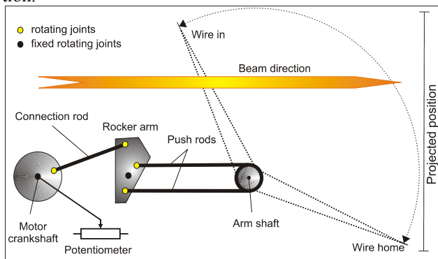
Figure 4: Schematic of a wire movement.
