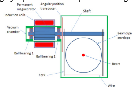
Figure 1: Simplified drawing of the future wire scanner. The green lines enclose the vacuum area.
