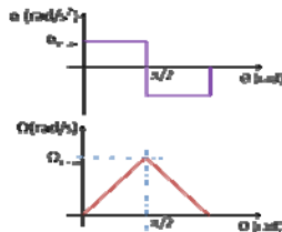
Figure 2: Theoretical angular acceleration (top) and angular speed (bottom) profile of the system.
