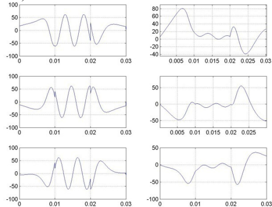
Figure 5: Simulated three phase voltage (left in volts) and current (right in amps) waveforms versus time in seconds.
