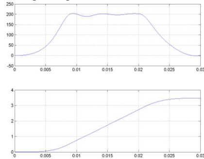
Figure 4: Simulated angular speed (top) and position (bottom) waveforms versus time in seconds.
