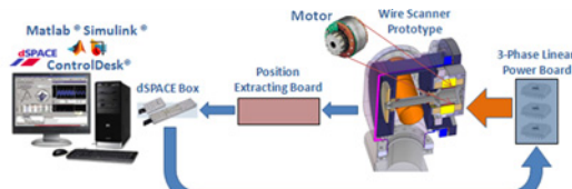
Figure 3: Synoptic view of the prototype.
