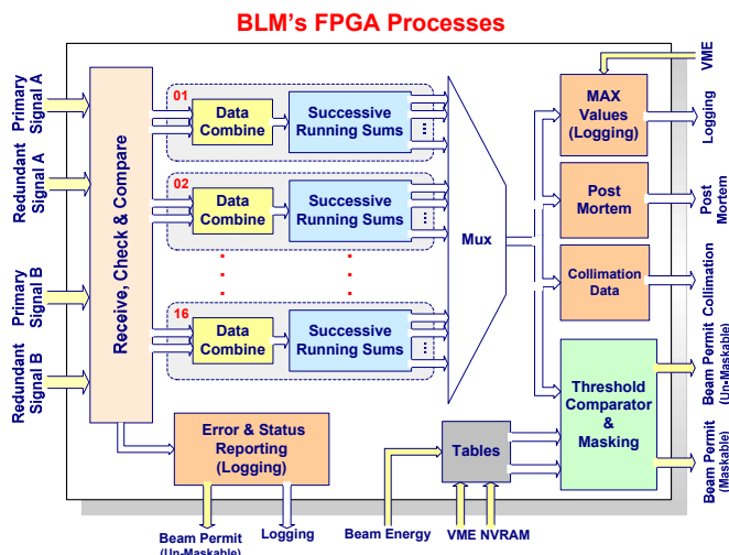
Figure 4: Overview of the Processes in the BLM's FPGA.
