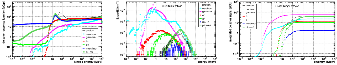
Figure 4: Left: GEANT4 simulated LHC BLM detector response functions for particle impact direction of 60^\circ . Center: Secondary particle fluence spectrum on the outside recorded in a 3.4 m long stripe, lethargy representation, MQY magnet, protons with 7 TeV impacting on the beam screen. Right: Integrated detector signal.
