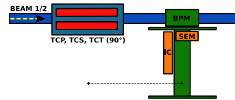
Figure 5: Structural view of a collimator (tilted at 90^\circ ) and its dedicated BLM detectors, an IC and a SEM, as mounted in the LHC cleaning insertions IR3 and IR7.
