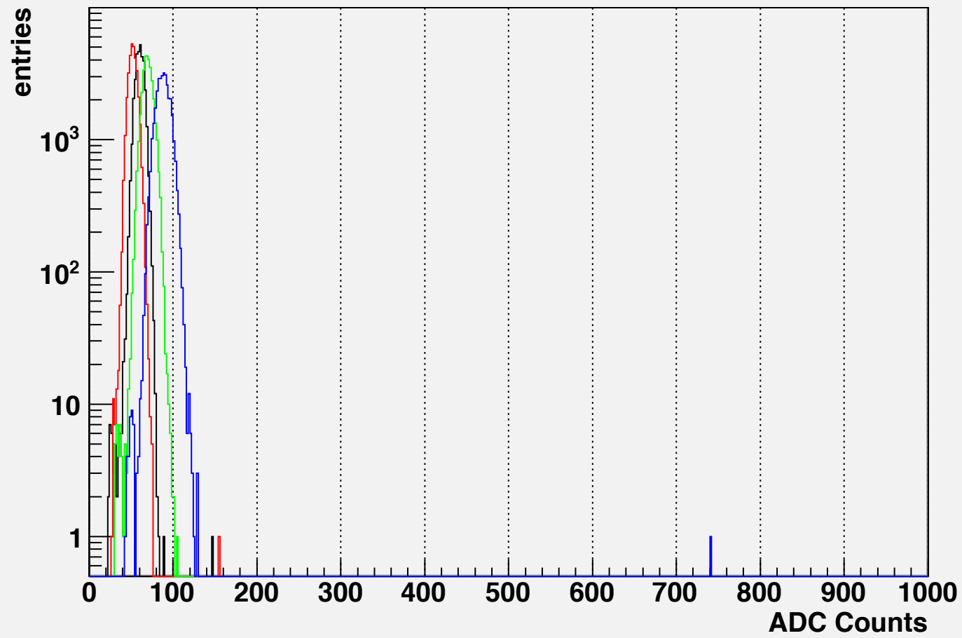
Signals in Direct dump monitors - Fill 1453
