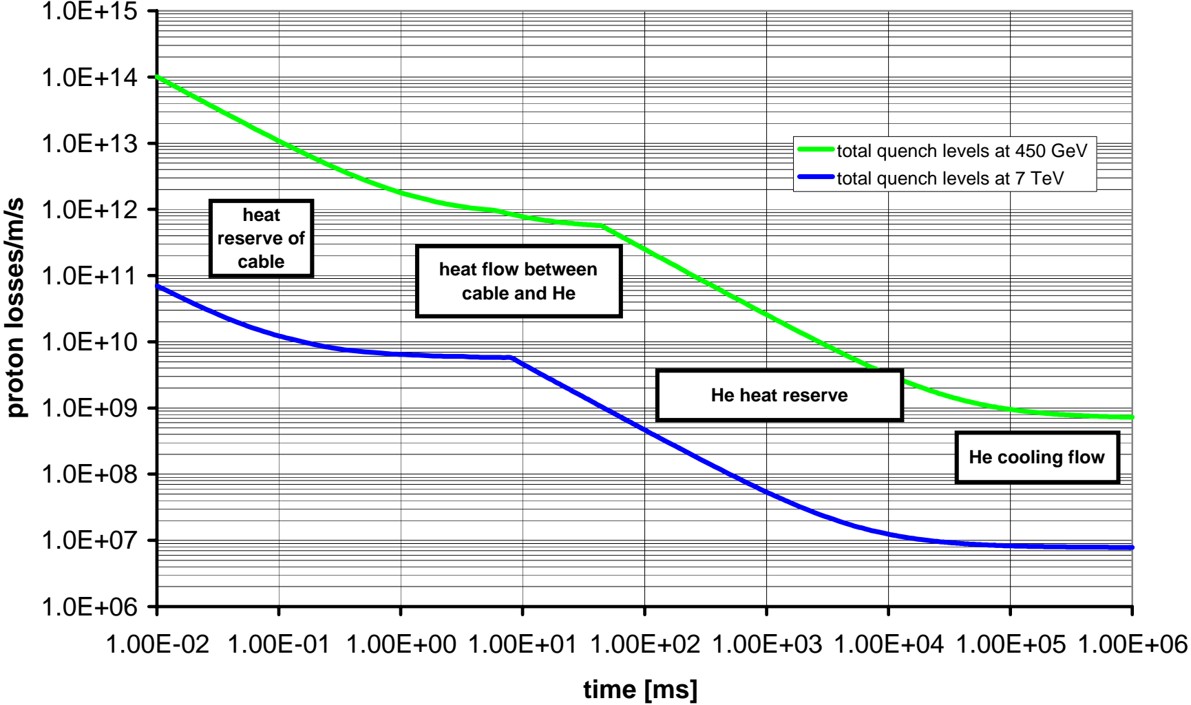
quench levels for LHC at 450 GeV and 7 TeV
