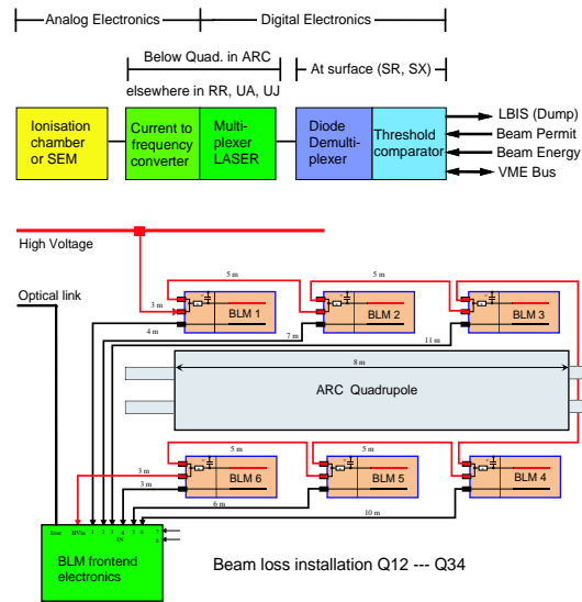
Figure 4: Schematic view of the signal transmission chain and the BLM installation around one arc quadrupole.
