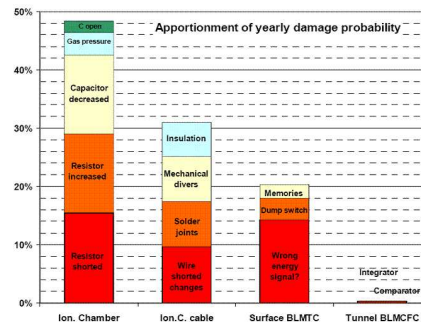
Figure 5: Relative probability of a system component being responsible for a damage to a LHC magnet in the case of a loss.
